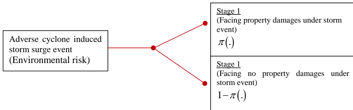
Figure 1: Probability Tree of a Sequence of Events
